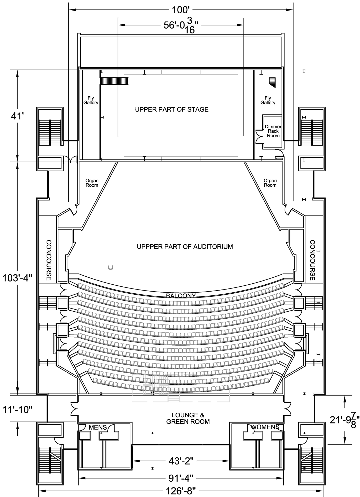
WILLIAMS AUDITORIUM SECOND FLOOR 646 SEATS
